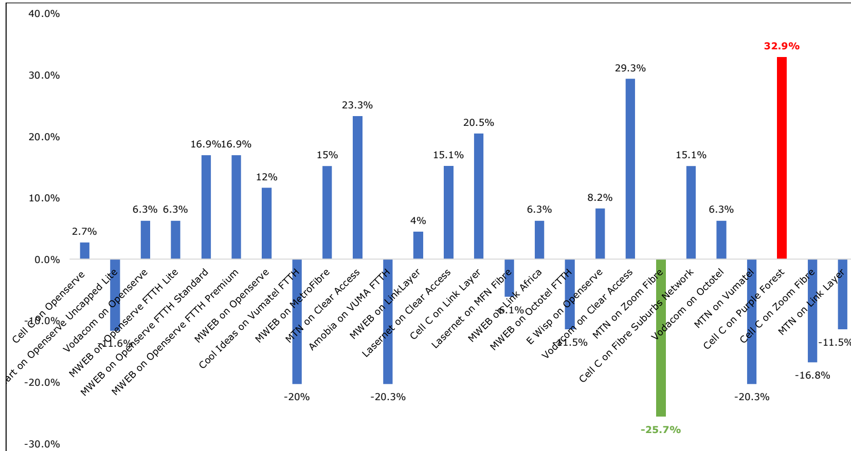
Figure 7: Percentage Deviation from the 25/25Mbps Average Price
